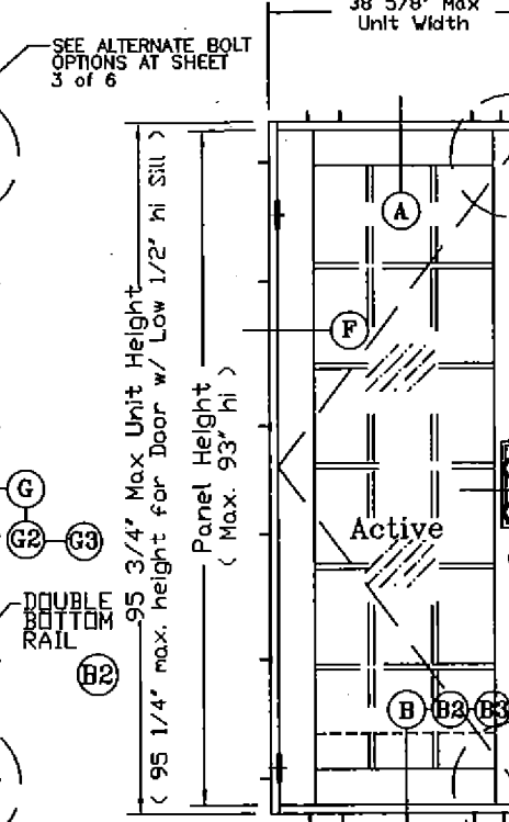
"X" ELEVATION
