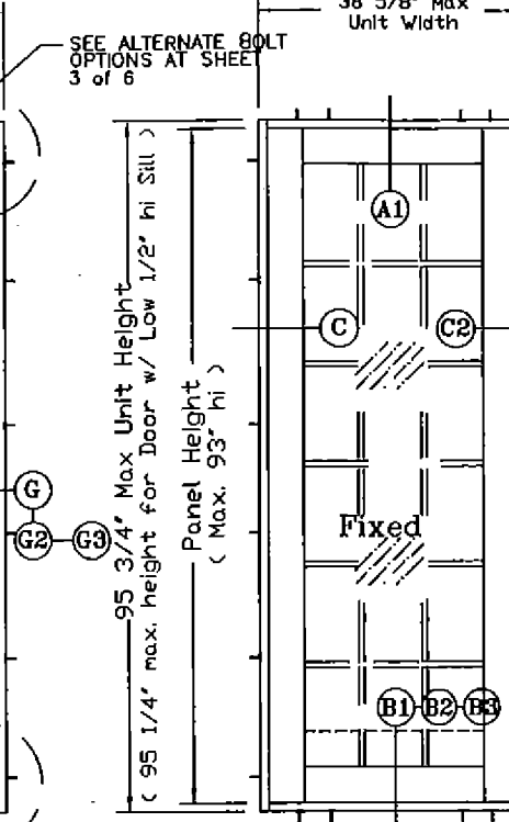
"O" ELEVATION
