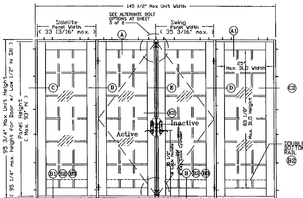
"OXO" ELEVATION
