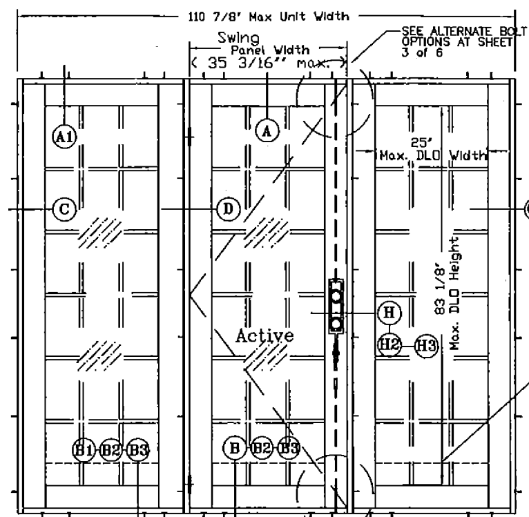
"OXO" ELEVATION
