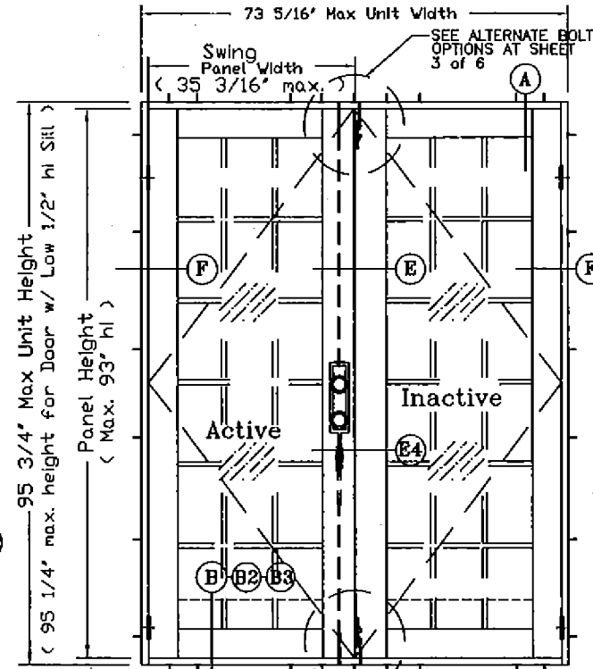
"XX" ELEVATION
