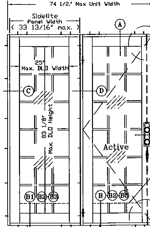
"OX" ELEVATION
